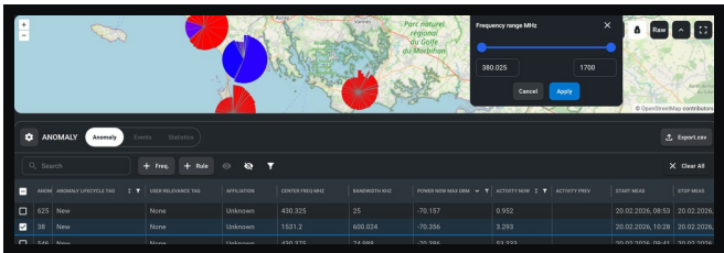
ANOMALY DETECTION ACROSS THE MONITORED BAND
