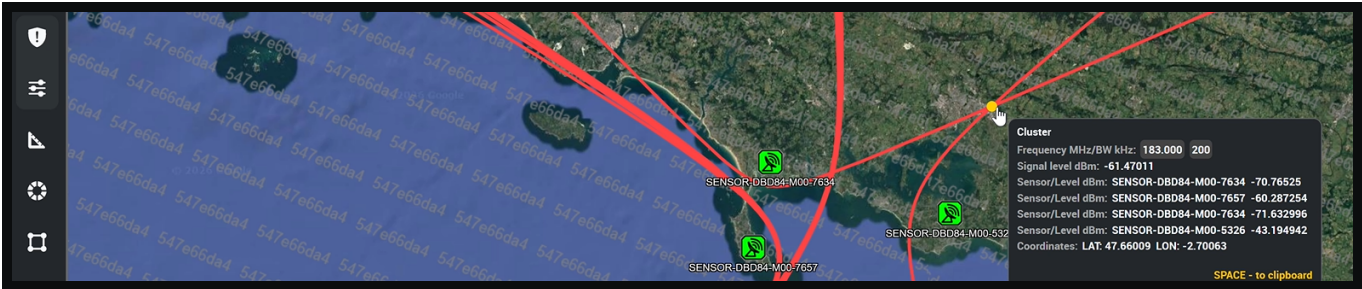
ELECTRONIC WARFARE MAP: TDOA LOCALISATION HYPERBOLAS AND CLUSTERISED TARGETS
